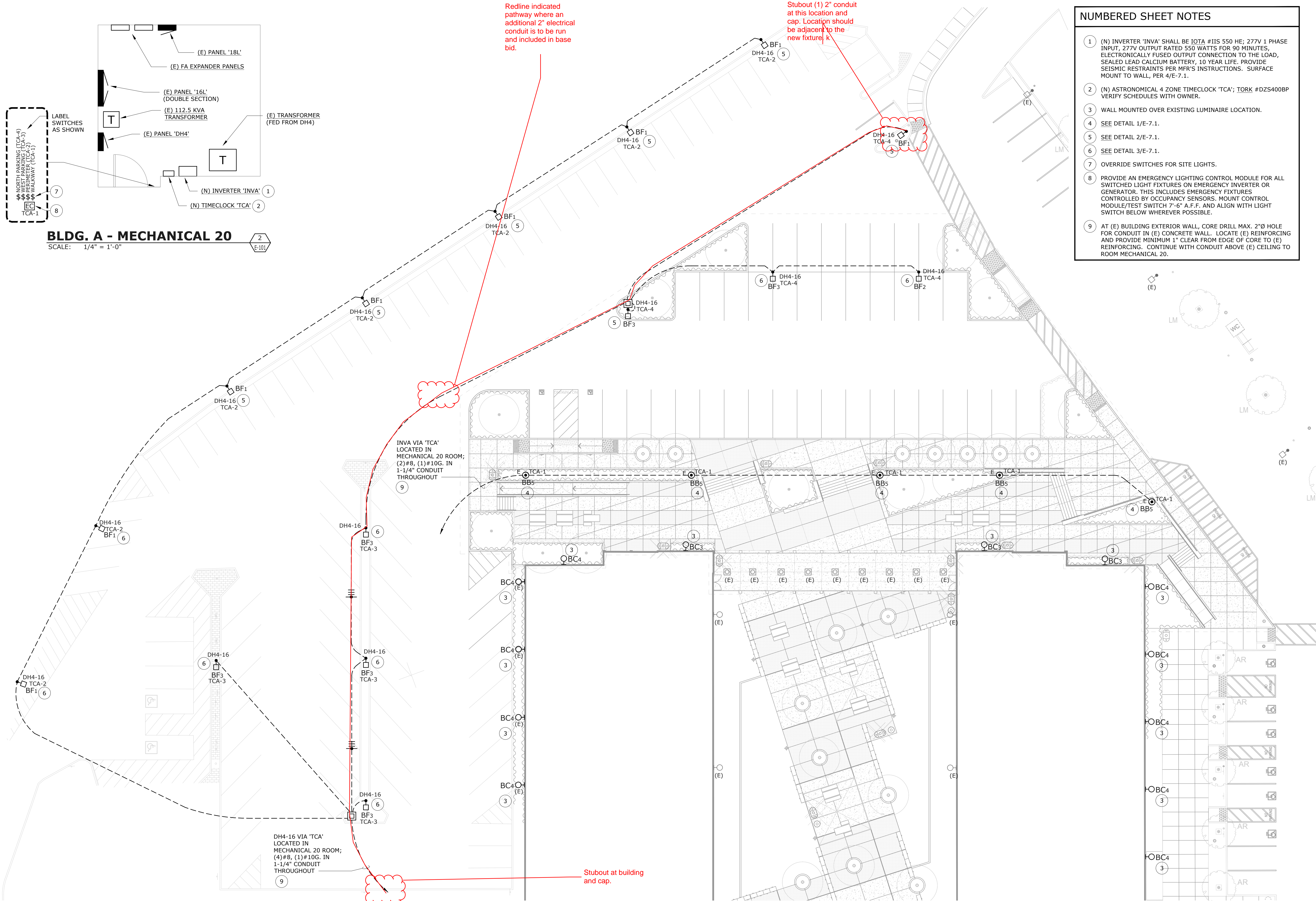
SITE PLAN - LIGHTING NORTH SCALE: 1/16" = 1'-0"
